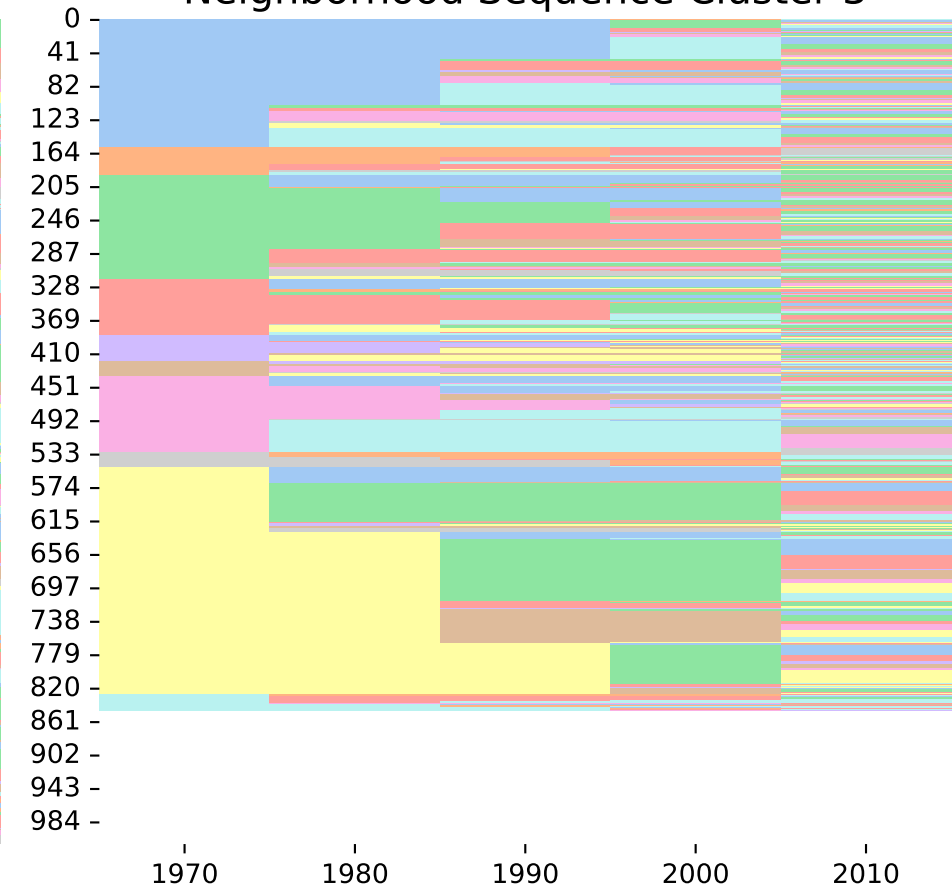
Neighborhood Sequence Cluster 3
